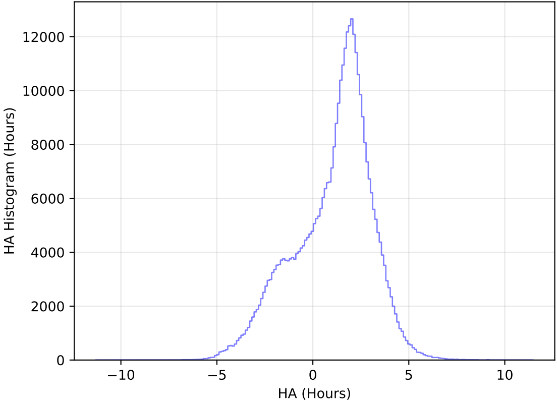
too_elab_heavy_r64_d3_griz_v3.4_10yrs WFD y band: HA Histogram
