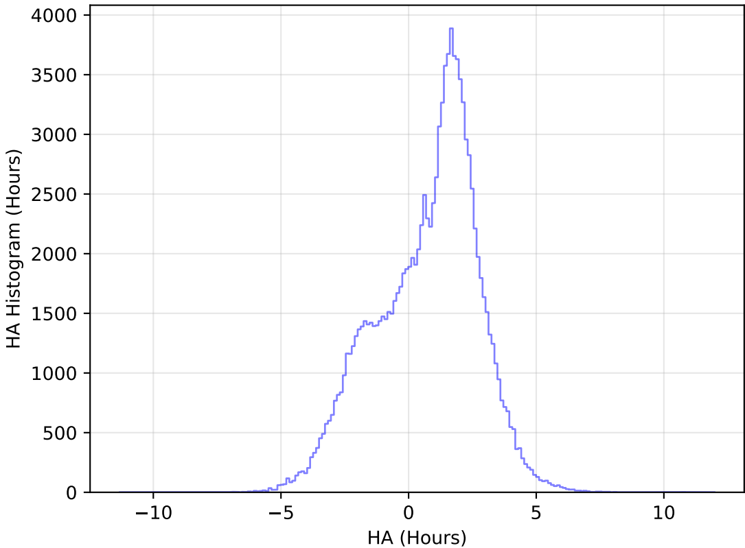
too_elab_heavy_r64_d3_griz_v3.4_10yrs WFD u band: HA Histogram
