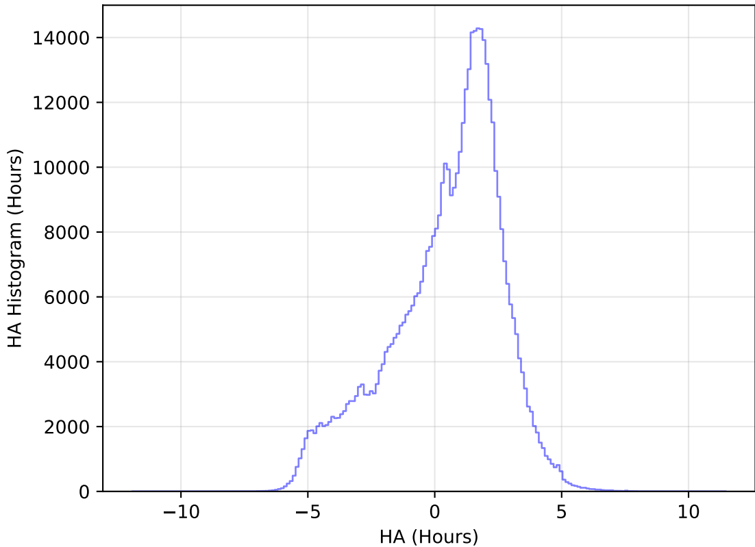
too_elab_heavy_r64_d3_griz_v3.4_10yrs WFD r band: HA Histogram
