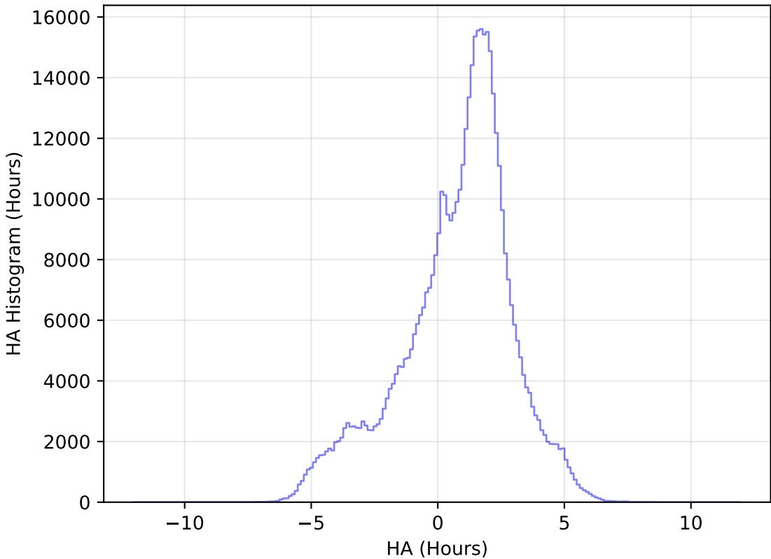
too_elab_heavy_r64_d3_griz_v3.4_10yrs WFD i band: HA Histogram
