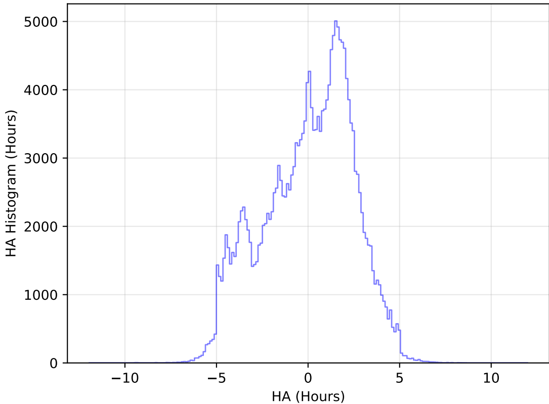
too_elab_heavy_r64_d3_griz_v3.4_10yrs WFD g band: HA Histogram
