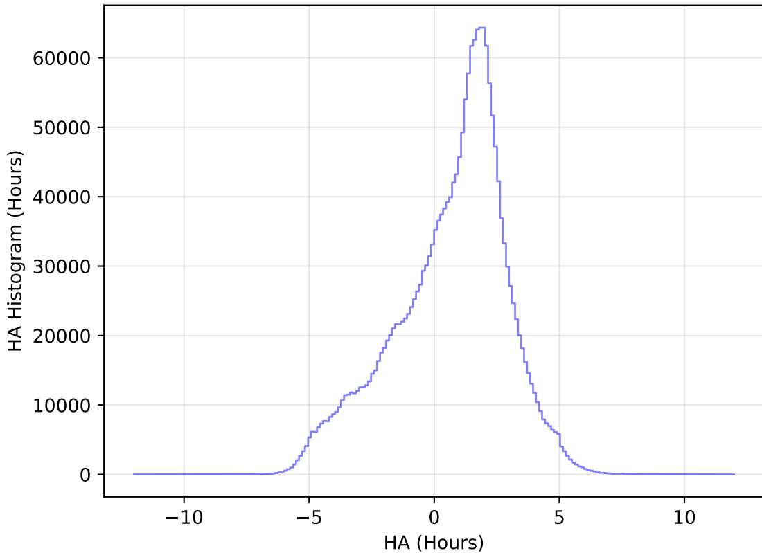
too_elab_heavy_r64_d3_griz_v3.4_10yrs WFD all bands: HA Histogram
