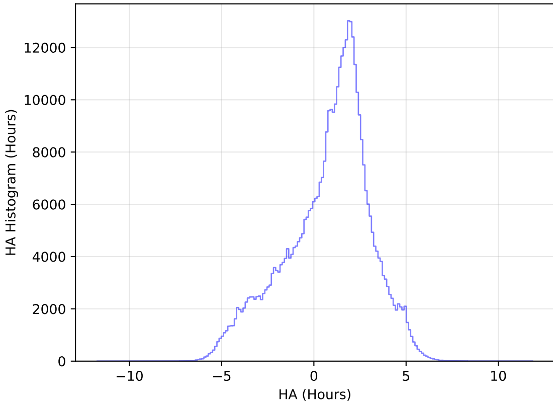
too_elab_heavy_r64_d3_griz_v3.4_10yrs All sky z band: HA Histogram
