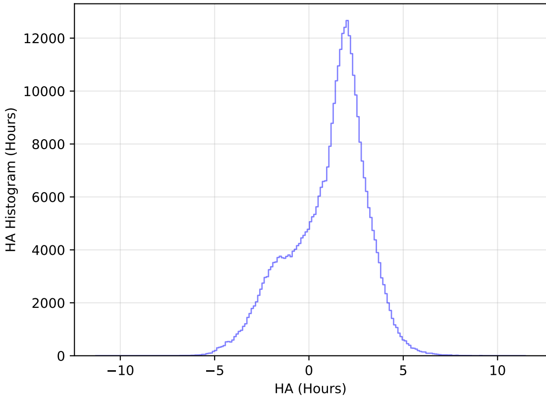
too_elab_heavy_r64_d3_griz_v3.4_10yrs All sky y band: HA Histogram
