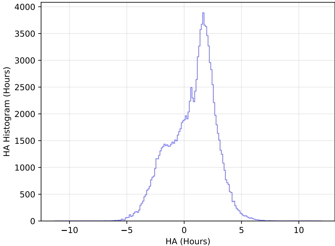
too_elab_heavy_r64_d3_griz_v3.4_10yrs All sky u band: HA Histogram
