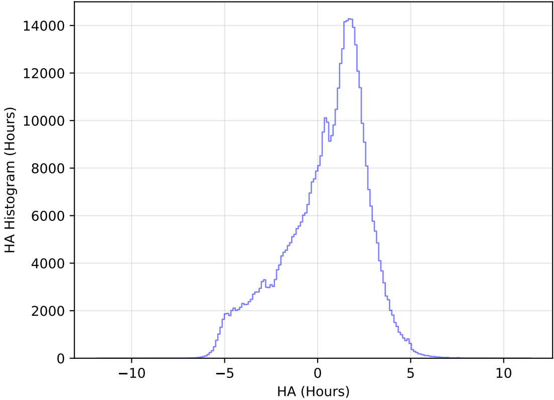
too_elab_heavy_r64_d3_griz_v3.4_10yrs All sky r band: HA Histogram
