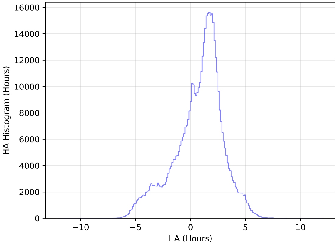
too_elab_heavy_r64_d3_griz_v3.4_10yrs All sky i band: HA Histogram
