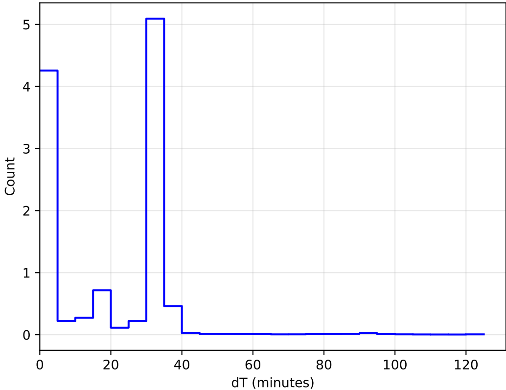
too_elab_heavy_r64_d3_griz_v3.4_10yrs WFD: DeltaT Histogram
