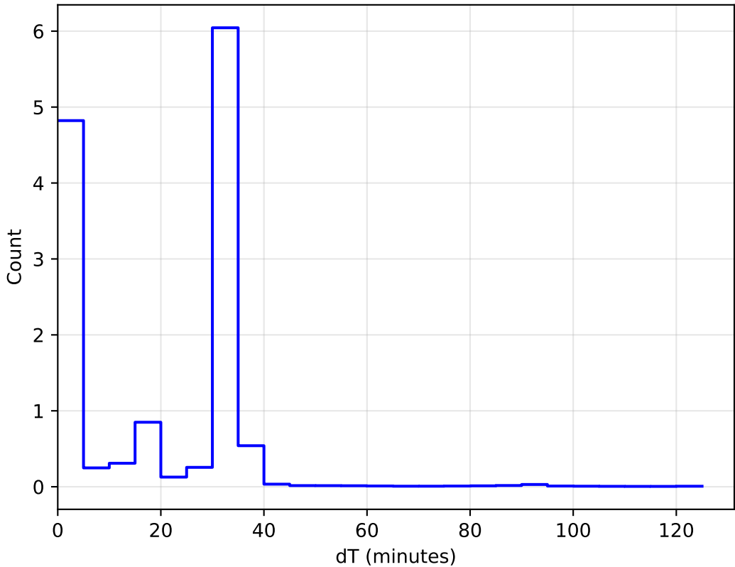
too_elab_heavy_r64_d3_griz_v3.4_10yrs All sky: DeltaT Histogram 1e6
