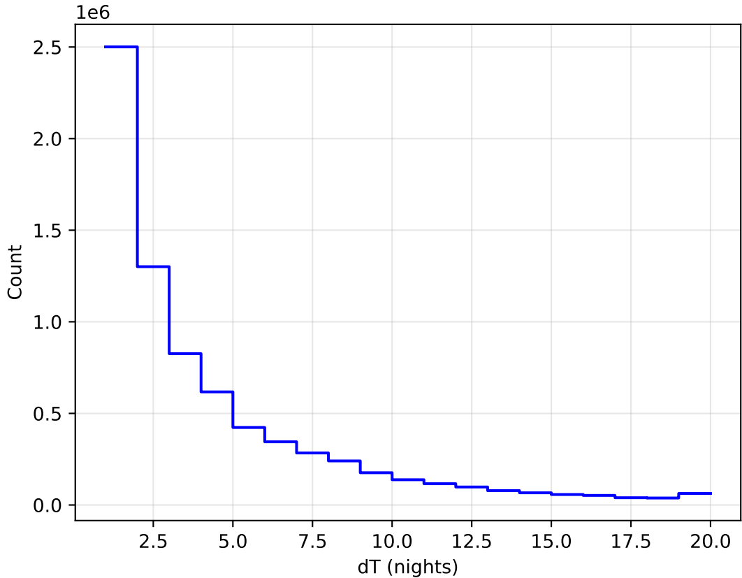
too_elab_heavy_r64_d3_griz_v3.4_10yrs WFD all bands: DeltaNight Histogram
