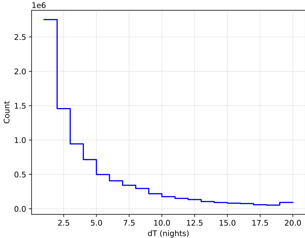
too_elab_heavy_r64_d3_griz_v3.4_10yrs All sky all bands: DeltaNight Histogram
