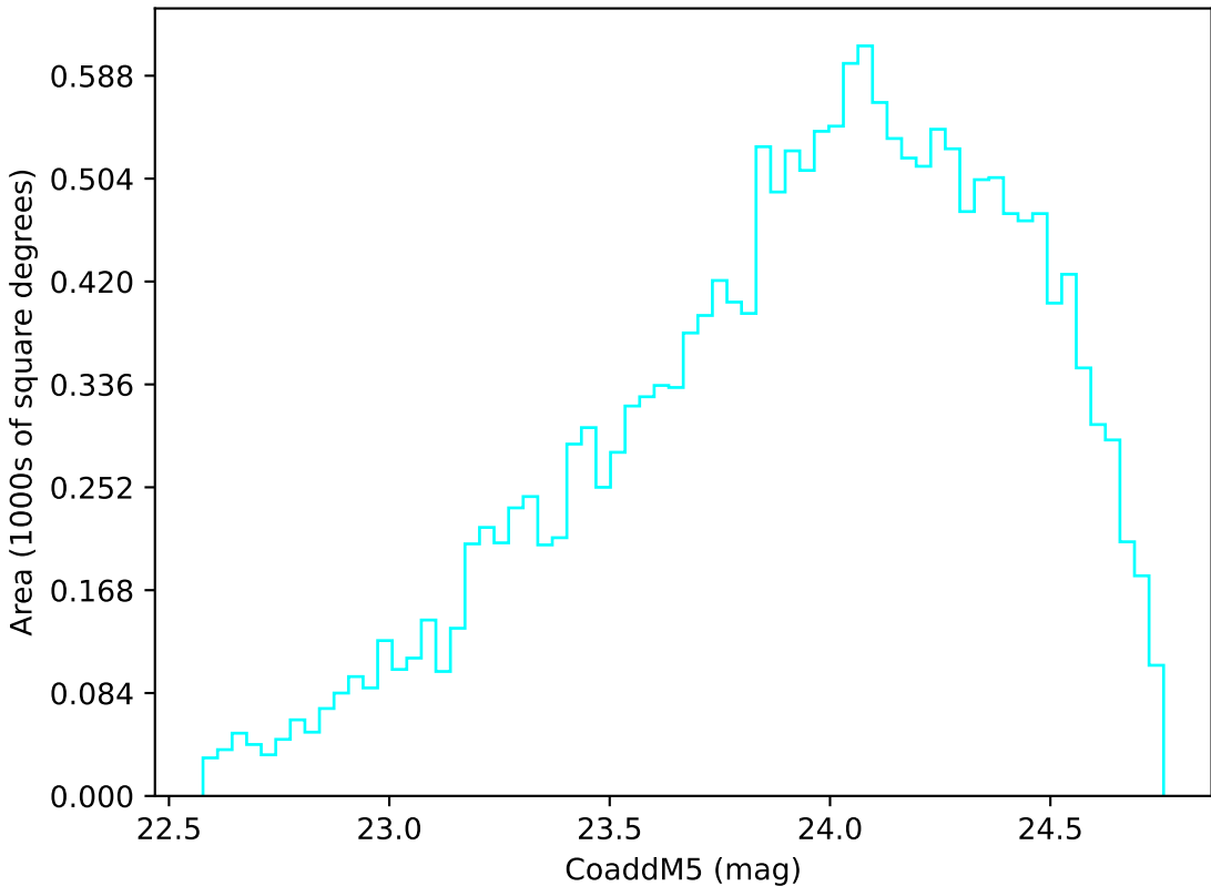
too_elab_heavy_r64_d3_griz_v3.4_10yrs Yr 3-4 u band: CoaddM5
