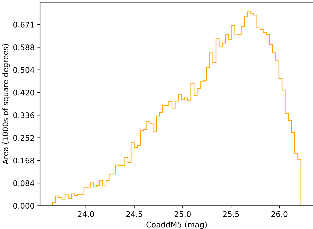
too_elab_heavy_r64_d3_griz_v3.4_10yrs Yr 3-4 r band: CoaddM5
