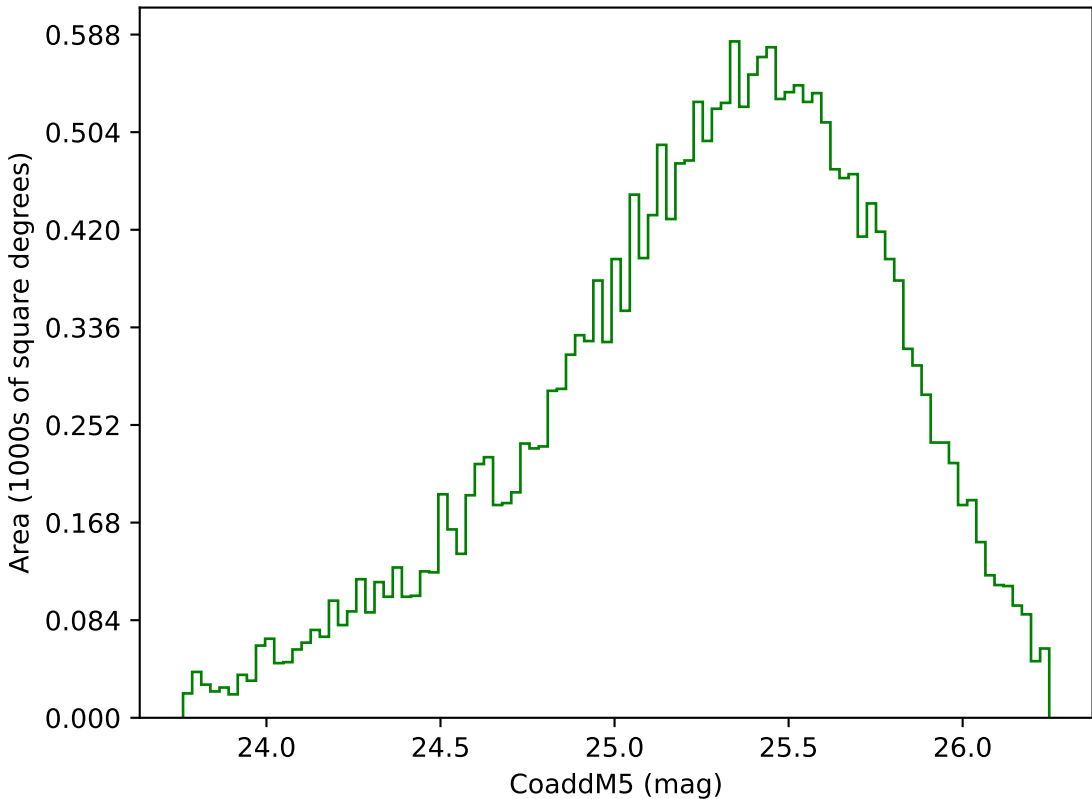
too_elab_heavy_r64_d3_griz_v3.4_10yrs Yr 3-4 g band: CoaddM5
