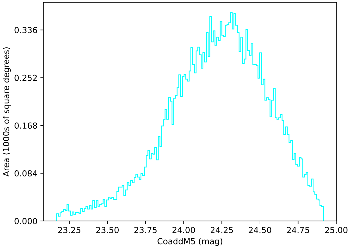
too_elab_heavy_r64_d3_griz_v3.4_10yrs Yr 1 u band: CoaddM5
