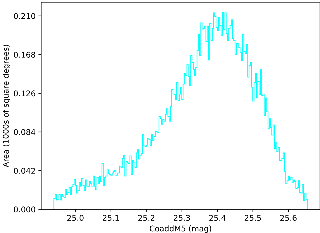
too_elab_heavy_r64_d3_griz_v3.4_10yrs WFD u band: CoaddM5
