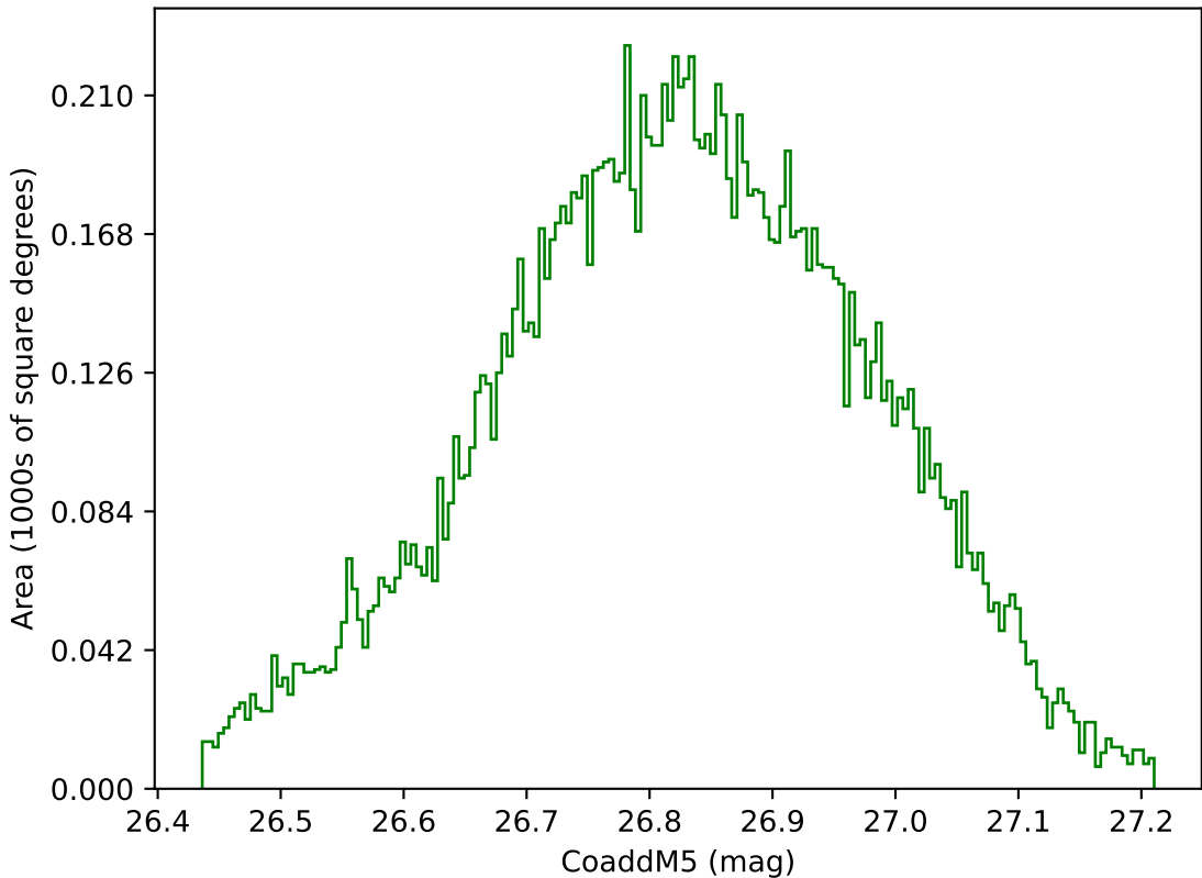
too_elab_heavy_r64_d3_griz_v3.4_10yrs WFD g band: CoaddM5
