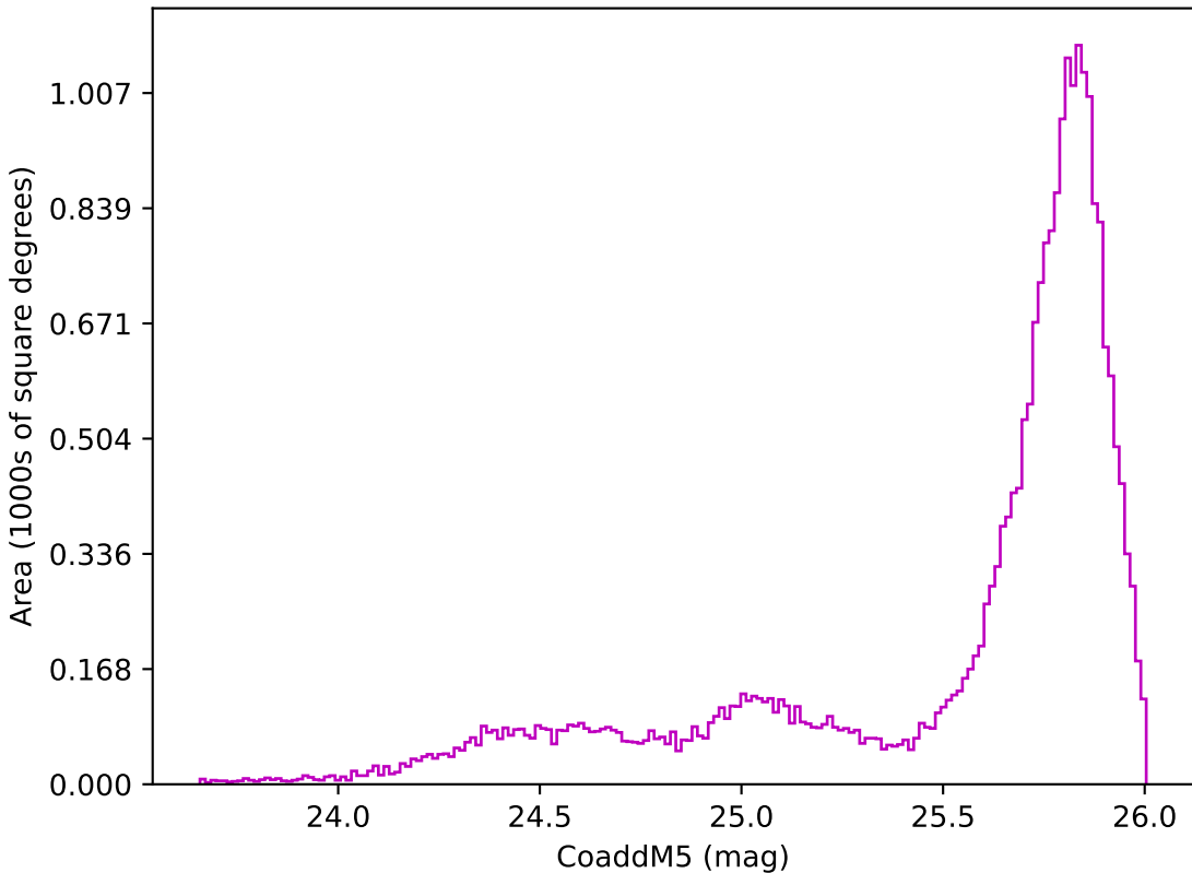
too_elab_heavy_r64_d3_griz_v3.4_10yrs All sky z band: CoaddM5
