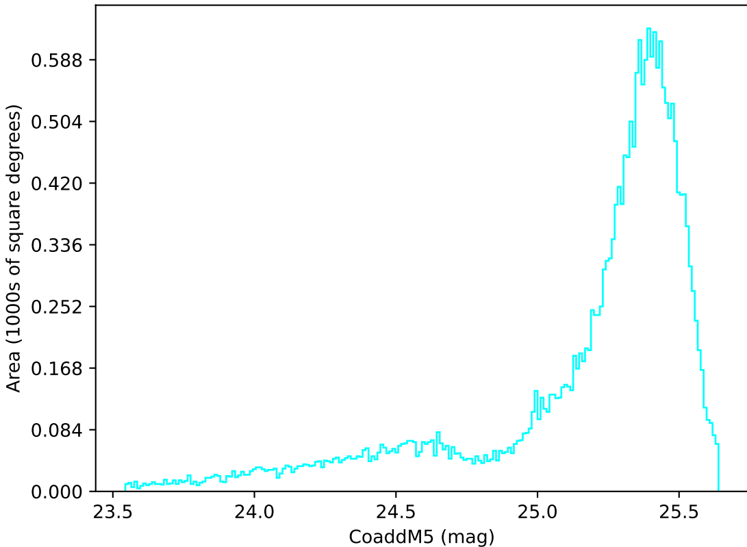
too_elab_heavy_r64_d3_griz_v3.4_10yrs All sky u band: CoaddM5
