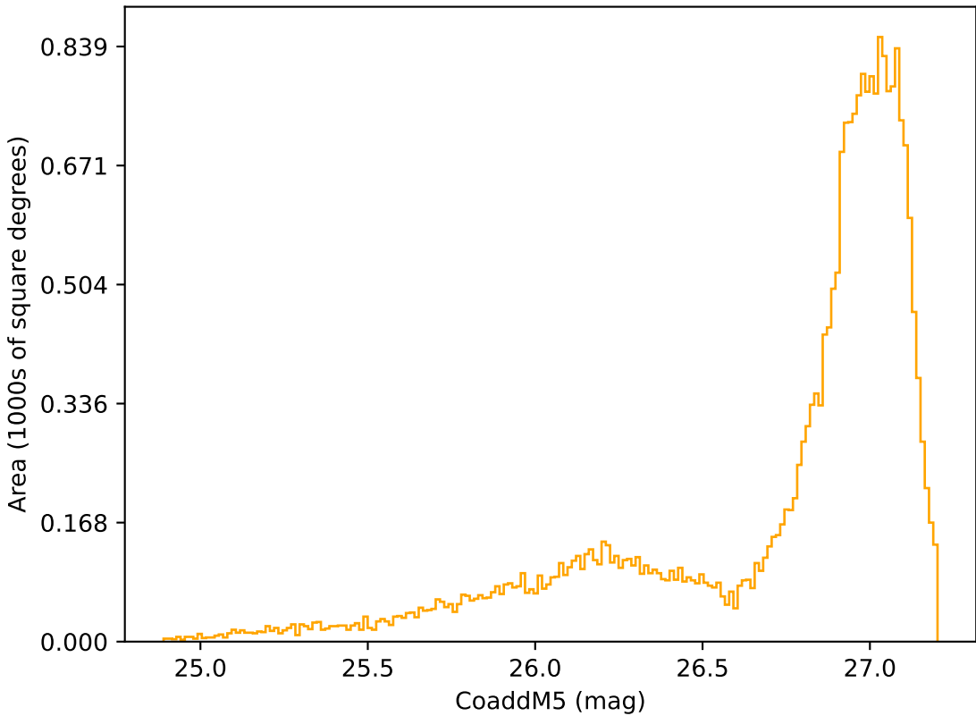
too_elab_heavy_r64_d3_griz_v3.4_10yrs All sky r band: CoaddM5
