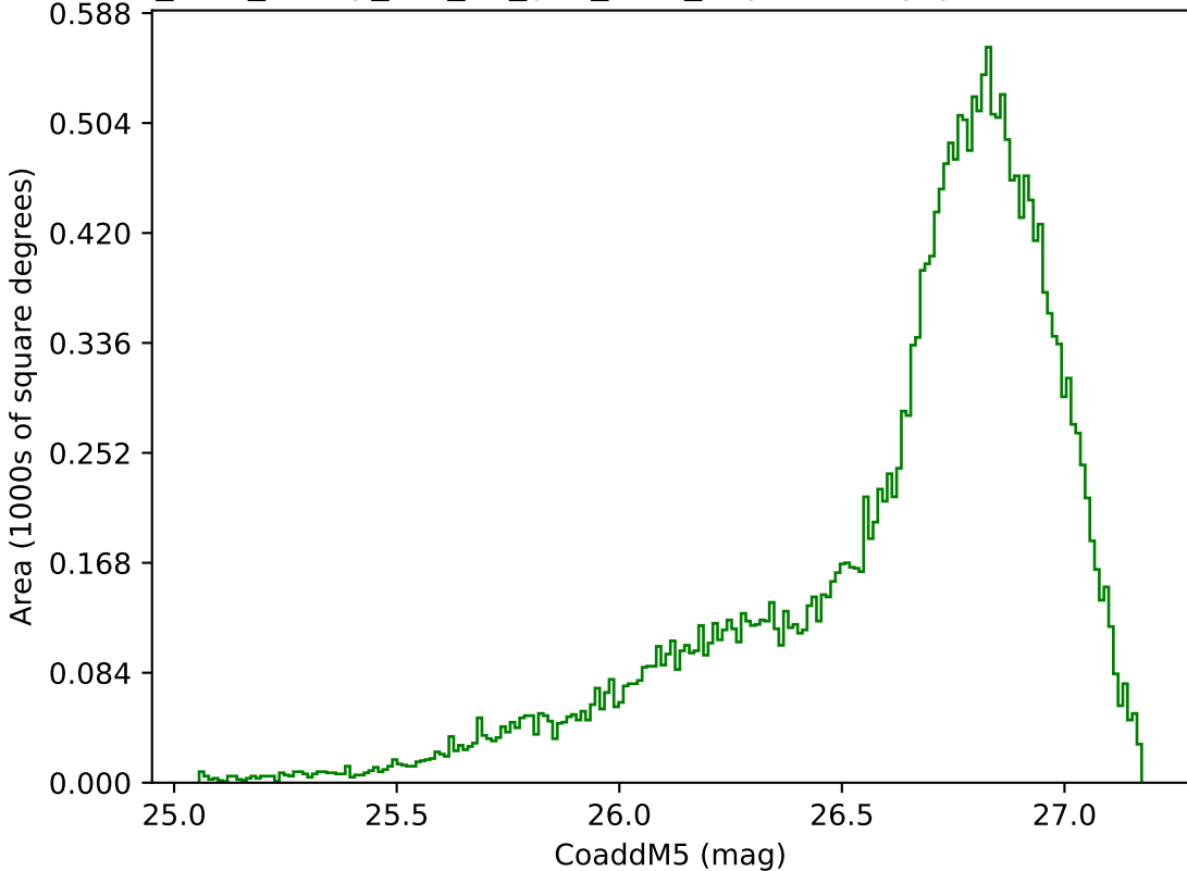
too_elab_heavy_r64_d3_griz_v3.4_10yrs All sky g band: CoaddM5
