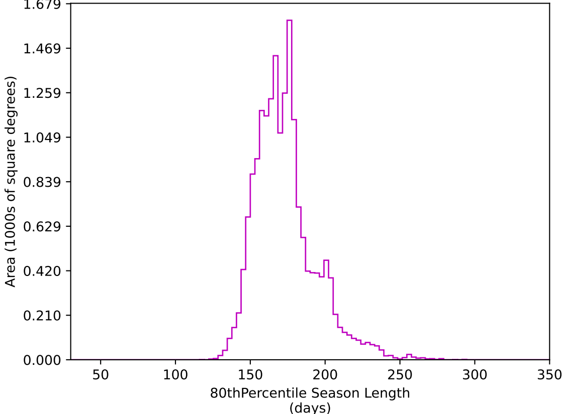
too_elab_heavy_r64_d3_griz_v3.4_10yrs WFD z band: 80thPercentile Season Length
