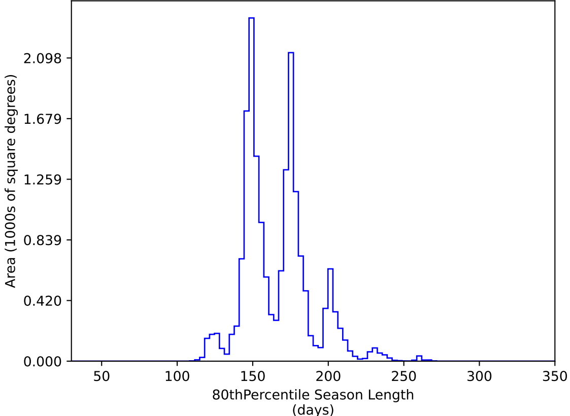
too_elab_heavy_r64_d3_griz_v3.4_10yrs WFD y band: 80thPercentile Season Length
