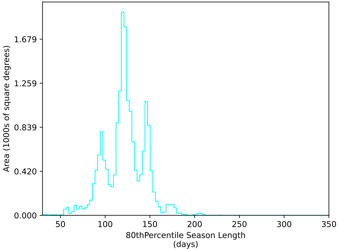
too_elab_heavy_r64_d3_griz_v3.4_10yrs WFD u band: 80thPercentile Season Length
