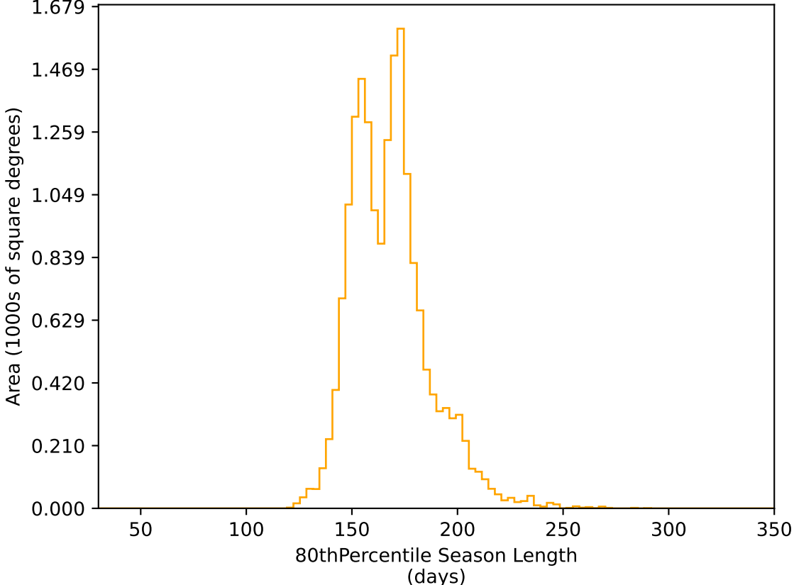
too_elab_heavy_r64_d3_griz_v3.4_10yrs WFD r band: 80thPercentile Season Length
