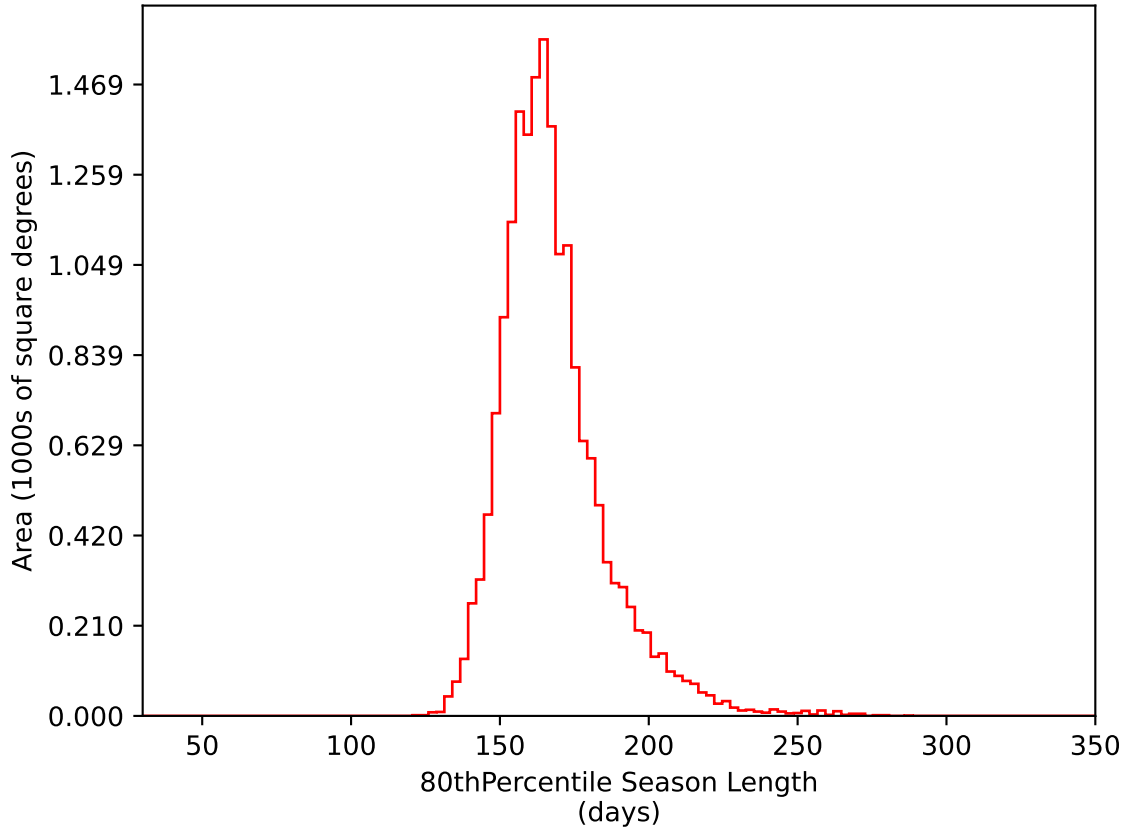
too_elab_heavy_r64_d3_griz_v3.4_10yrs WFD i band: 80thPercentile Season Length
