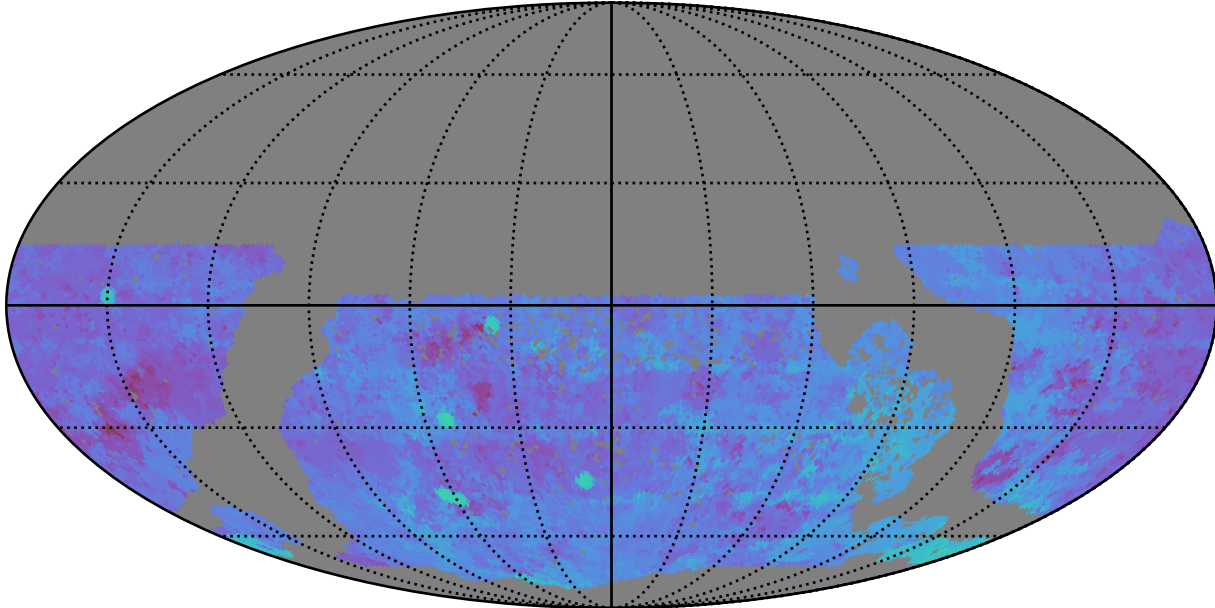
too_elab_heavy_r64_d3_griz_v3.4_10yrs WFD g band: 80thPercentile Season Length
