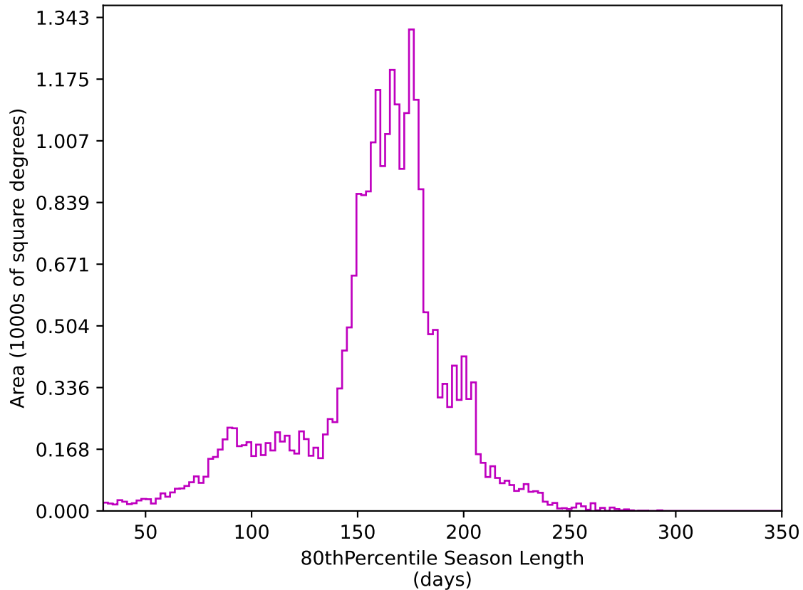
too_elab_heavy_r64_d3_griz_v3.4_10yrs All sky z band: 80thPercentile Season Length
