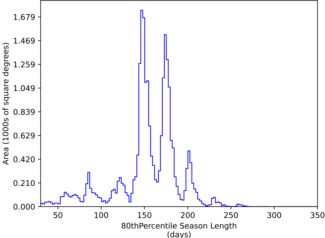
too_elab_heavy_r64_d3_griz_v3.4_10yrs All sky y band: 80thPercentile Season Length
