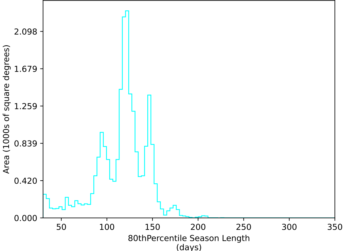
too_elab_heavy_r64_d3_griz_v3.4_10yrs All sky u band: 80thPercentile Season Length
