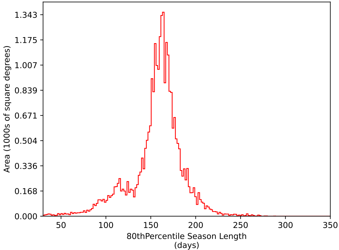
too_elab_heavy_r64_d3_griz_v3.4_10yrs All sky i band: 80thPercentile Season Length
