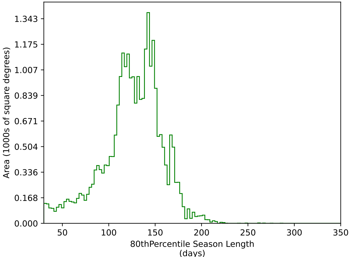
too_elab_heavy_r64_d3_griz_v3.4_10yrs All sky g band: 80thPercentile Season Length
