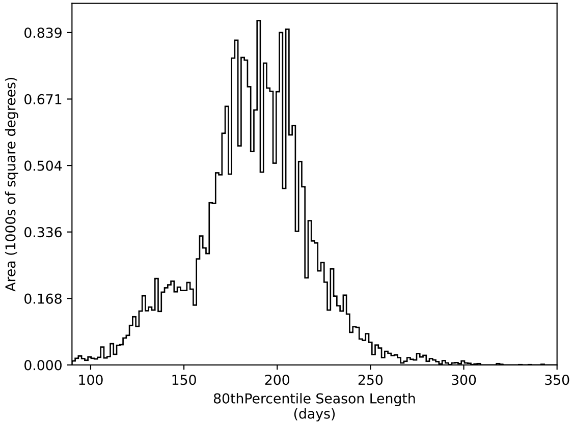
too_elab_heavy_r64_d3_griz_v3.4_10yrs All sky all bands: 80thPercentile Season Length
