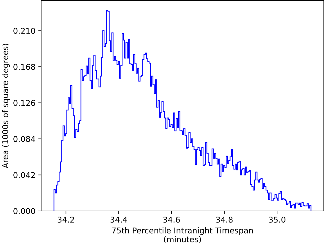
too_elab_heavy_r64_d3_griz_v3.4_10yrs WFD zy bands: 75th Percentile Intranight Timespan
