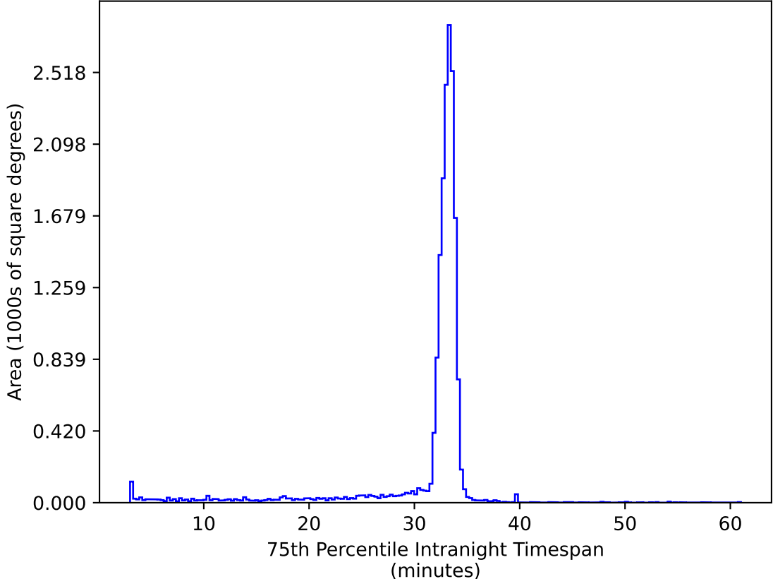
too_elab_heavy_r64_d3_griz_v3.4_10yrs WFD ug bands: 75th Percentile Intranight Timespan
