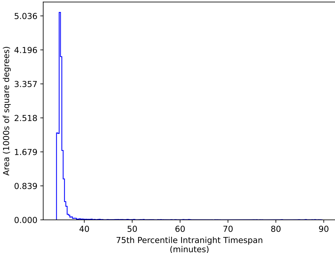
too_elab_heavy_r64_d3_griz_v3.4_10yrs WFD ri bands: 75th Percentile Intranight Timespan
