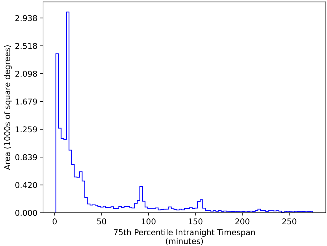
too_elab_heavy_r64_d3_griz_v3.4_10yrs WFD r band: 75th Percentile Intranight Timespan
