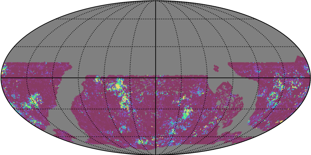
too_elab_heavy_r64_d3_griz_v3.4_10yrs WFD g band: 75th Percentile Intranight Timespan
