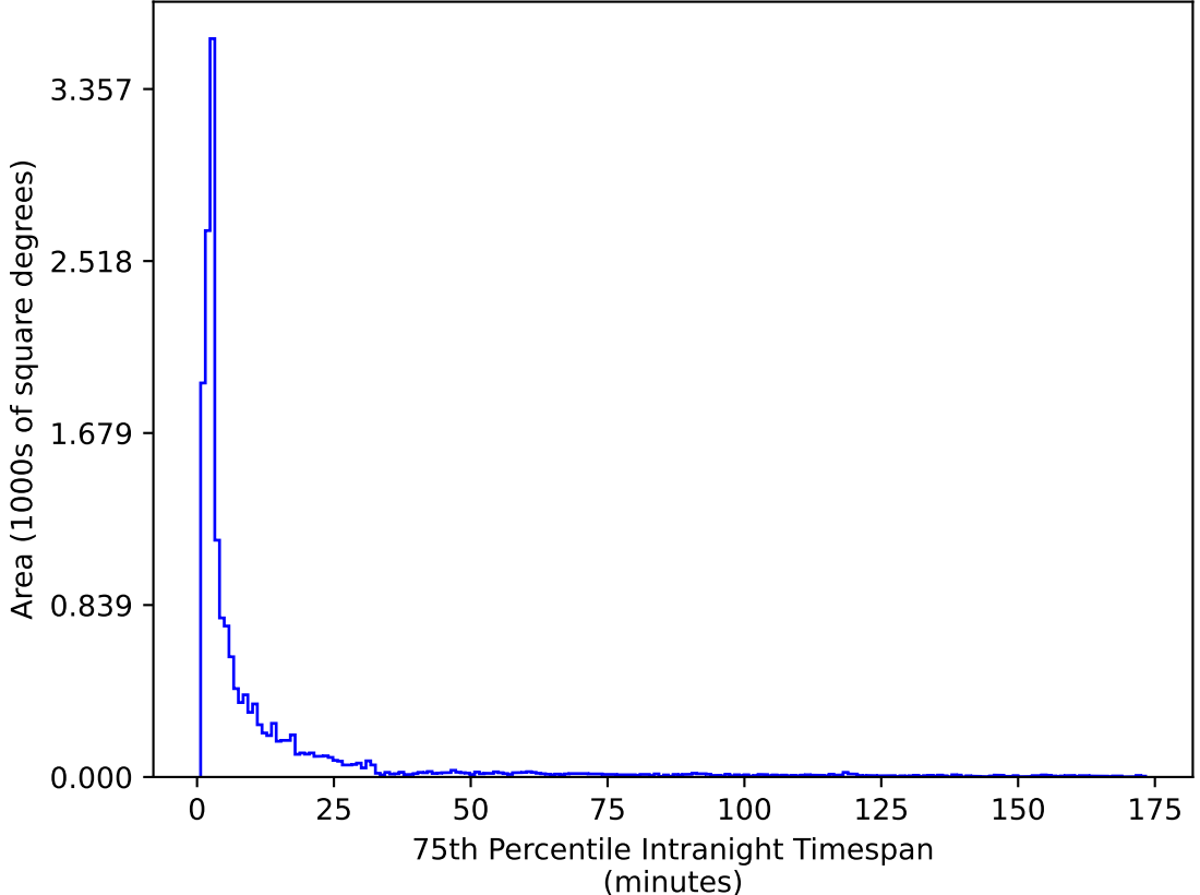
too_elab_heavy_r64_d3_griz_v3.4_10yrs WFD g band: 75th Percentile Intranight Timespan
