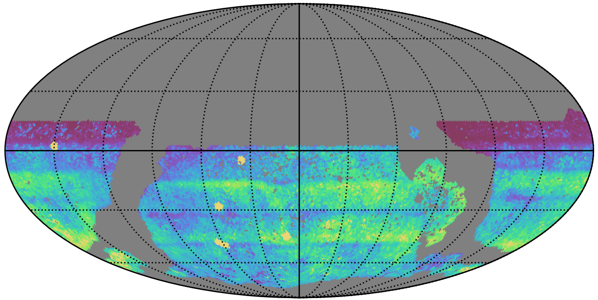
too_elab_heavy_r64_d3_griz_v3.4_10yrs WFD all bands: 75th Percentile Intranight Timespan
