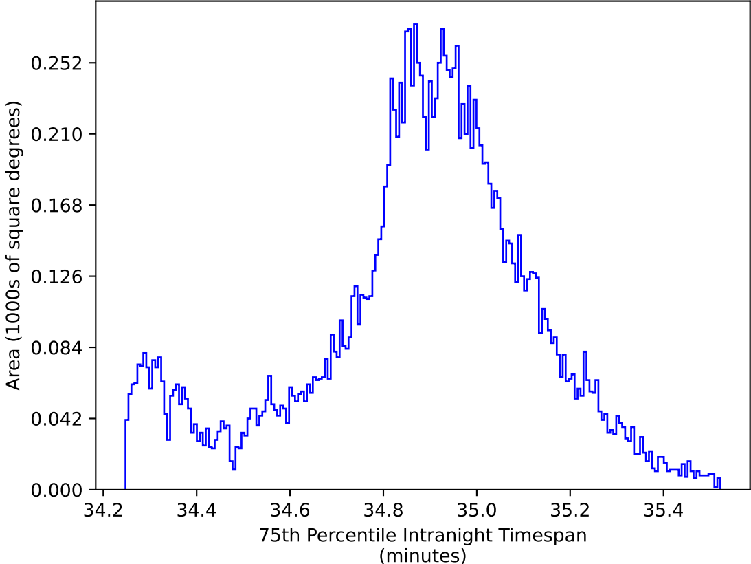
too_elab_heavy_r64_d3_griz_v3.4_10yrs WFD all bands: 75th Percentile Intranight Timespan
