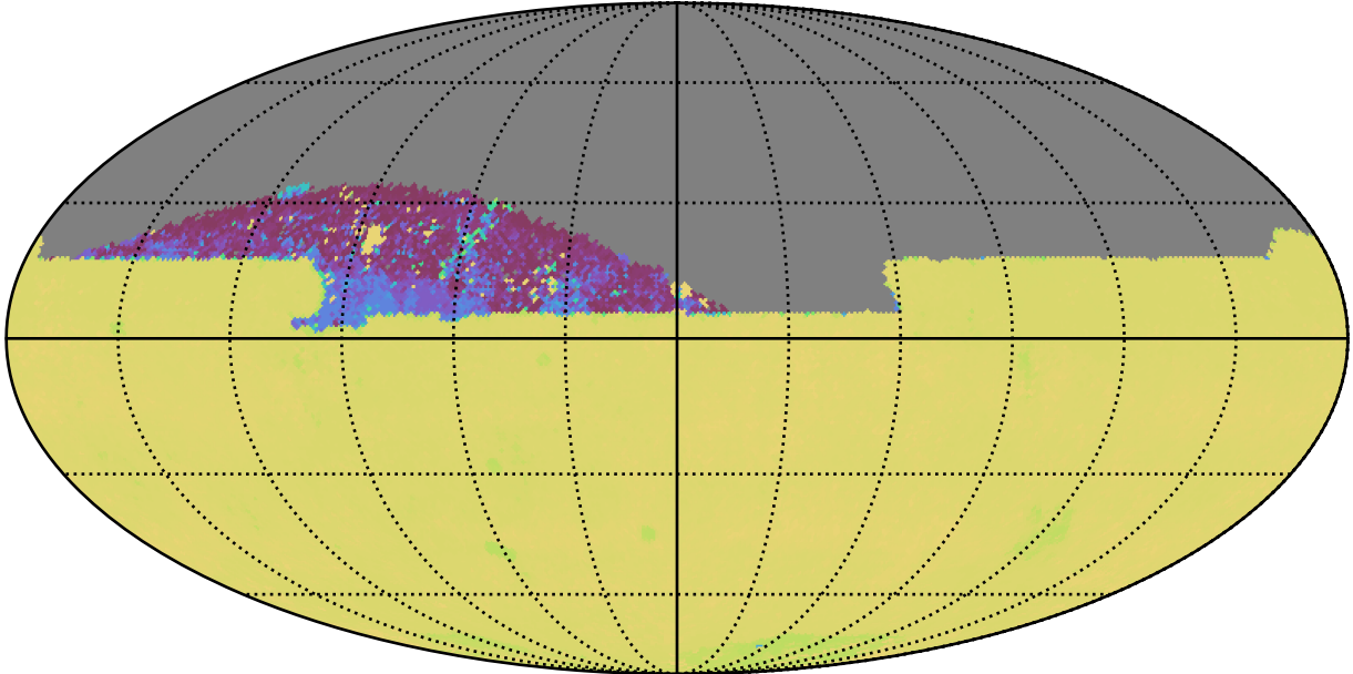
too_elab_heavy_r64_d3_griz_v3.4_10yrs All sky zy bands: 75th Percentile Intranight Timespan
