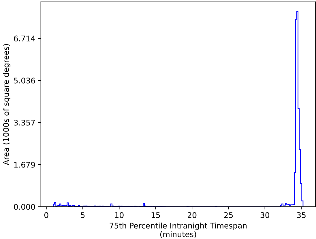
too_elab_heavy_r64_d3_griz_v3.4_10yrs All sky zy bands: 75th Percentile Intranight Timespan
