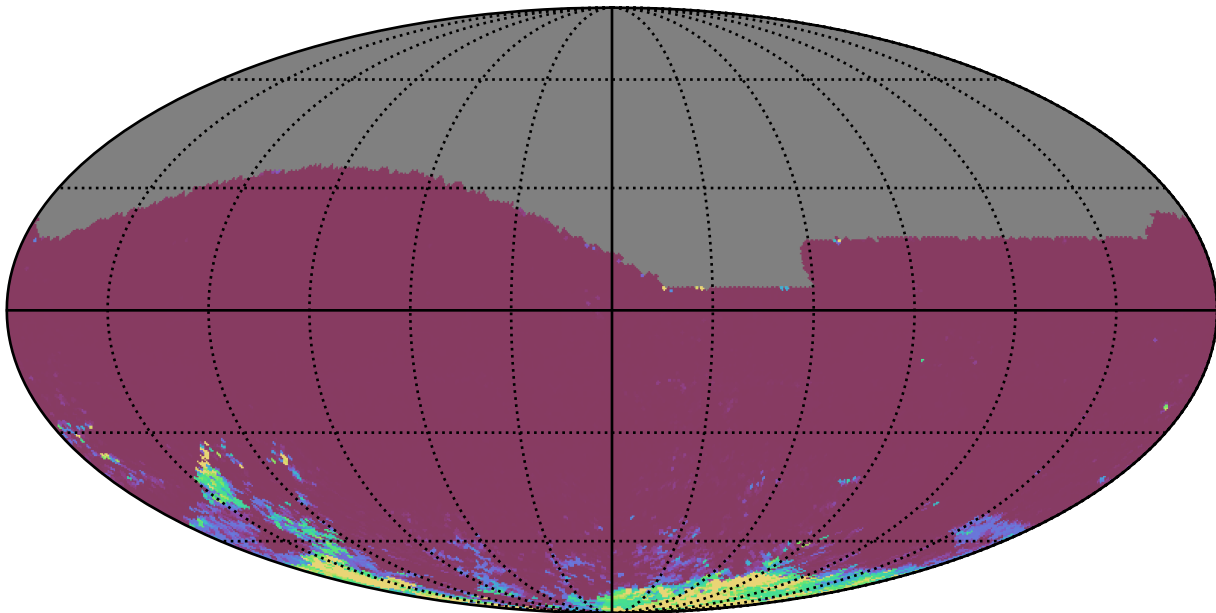
too_elab_heavy_r64_d3_griz_v3.4_10yrs All sky ri bands: 75th Percentile Intranight Timespan
