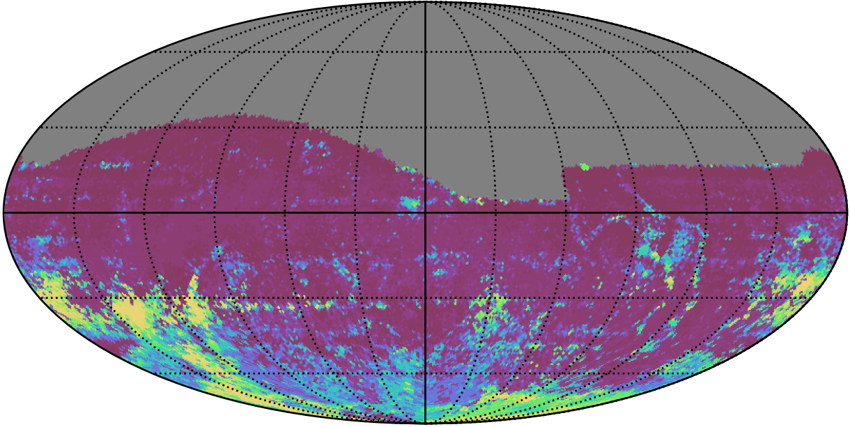
too_elab_heavy_r64_d3_griz_v3.4_10yrs All sky r band: 75th Percentile Intranight Timespan
