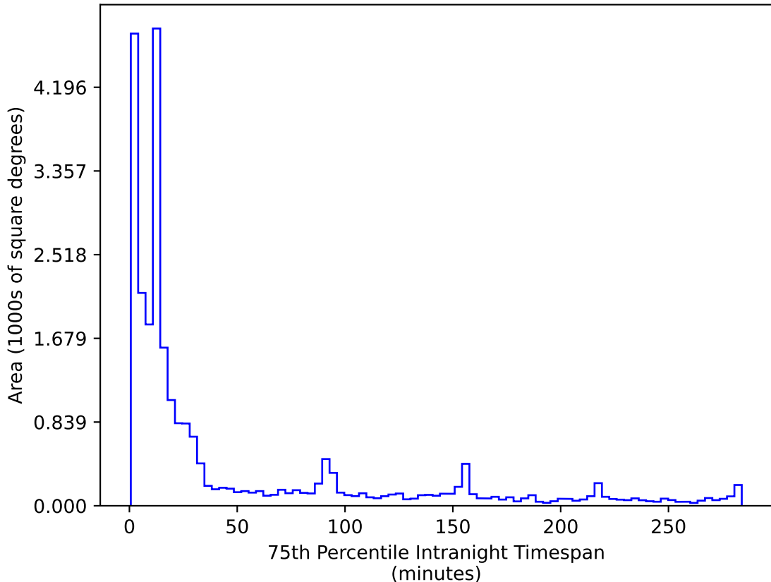
too_elab_heavy_r64_d3_griz_v3.4_10yrs All sky r band: 75th Percentile Intranight Timespan
